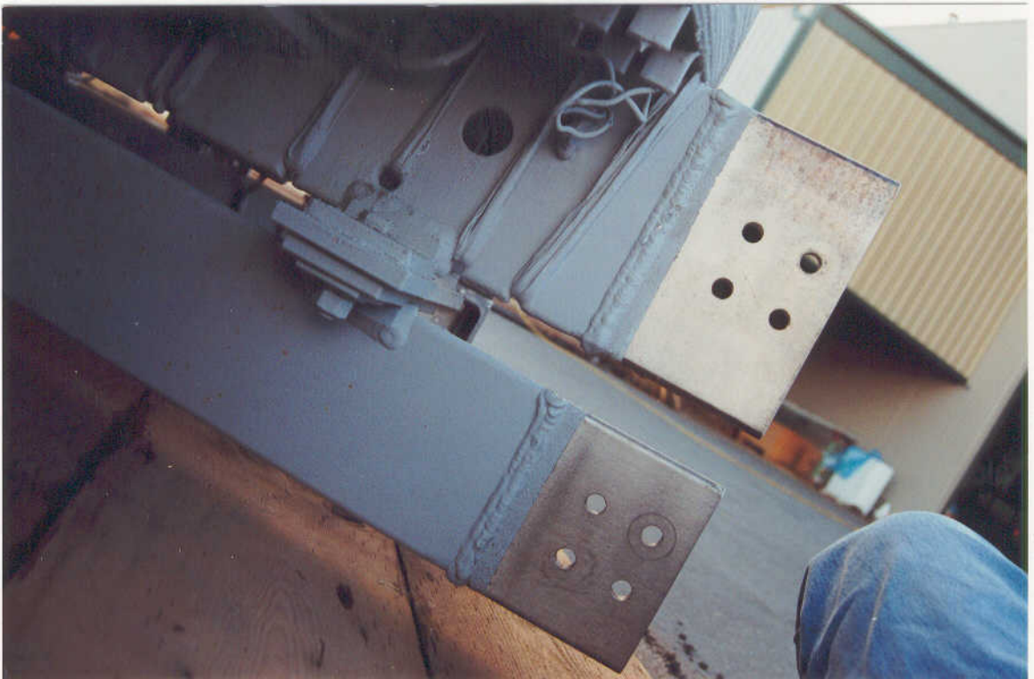
No. 23 - View of the bottom busbars. No evidence of physical damages were present.
